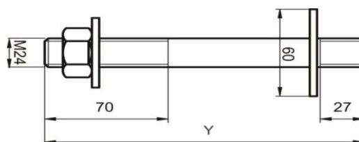
Skica 1: Opornica M24/Y; Y=145 mm
